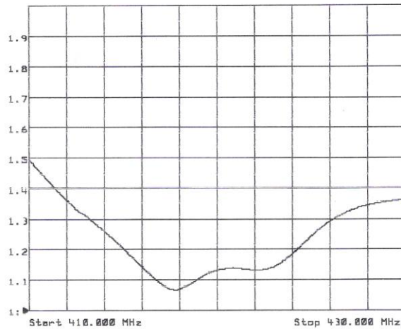
FREQUENCY vs VSWR CHART
