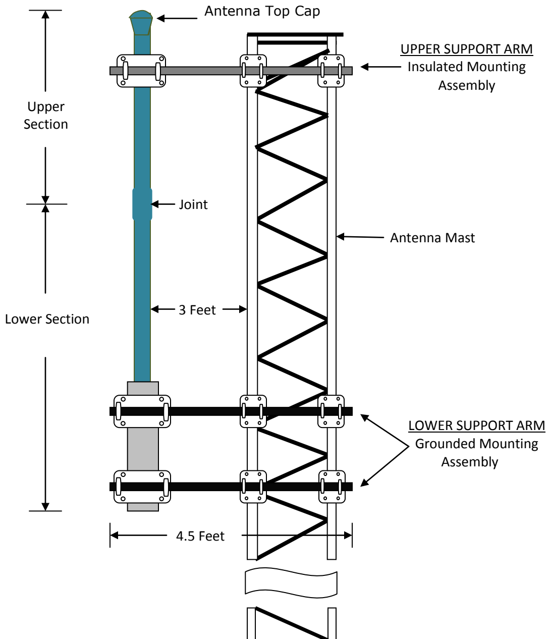
Installation Diagram of AC7-156-162 Collinear Antenna
